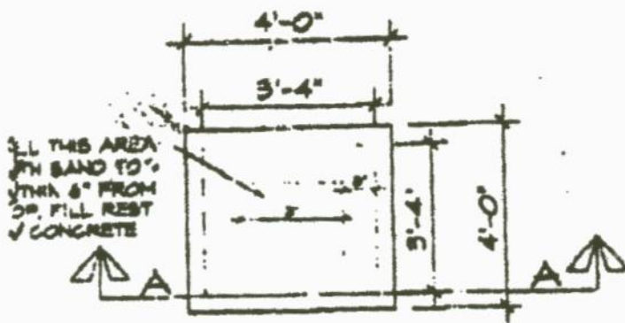
PLAN SCALE 1/2"=1'-0"
